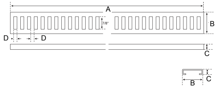
Drain Assembly
