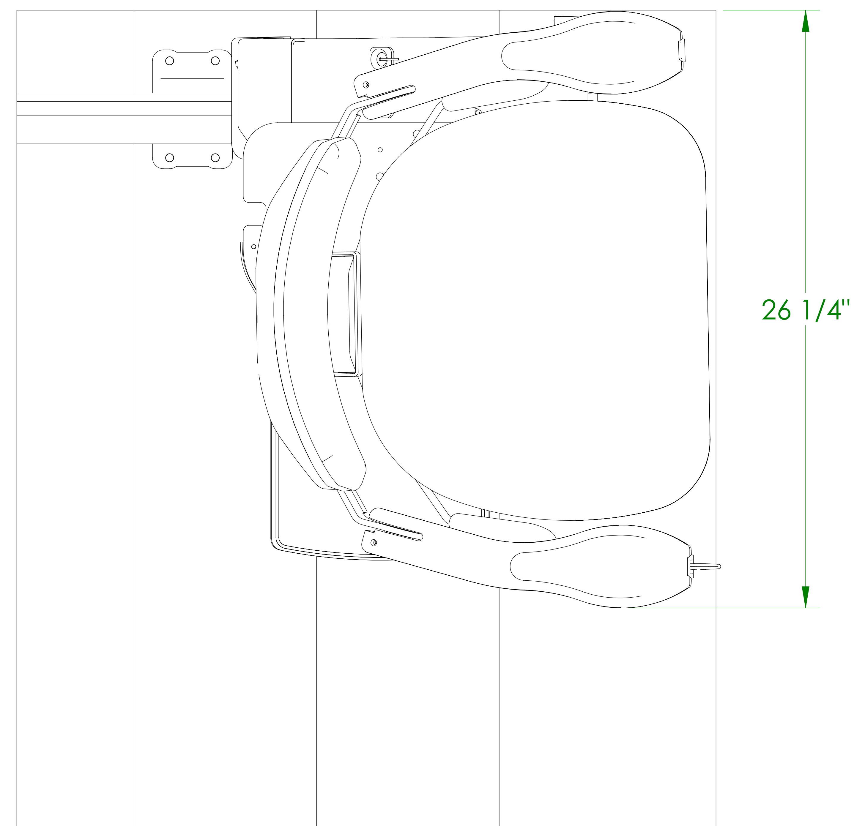
SEAT SWIVELED 90°
