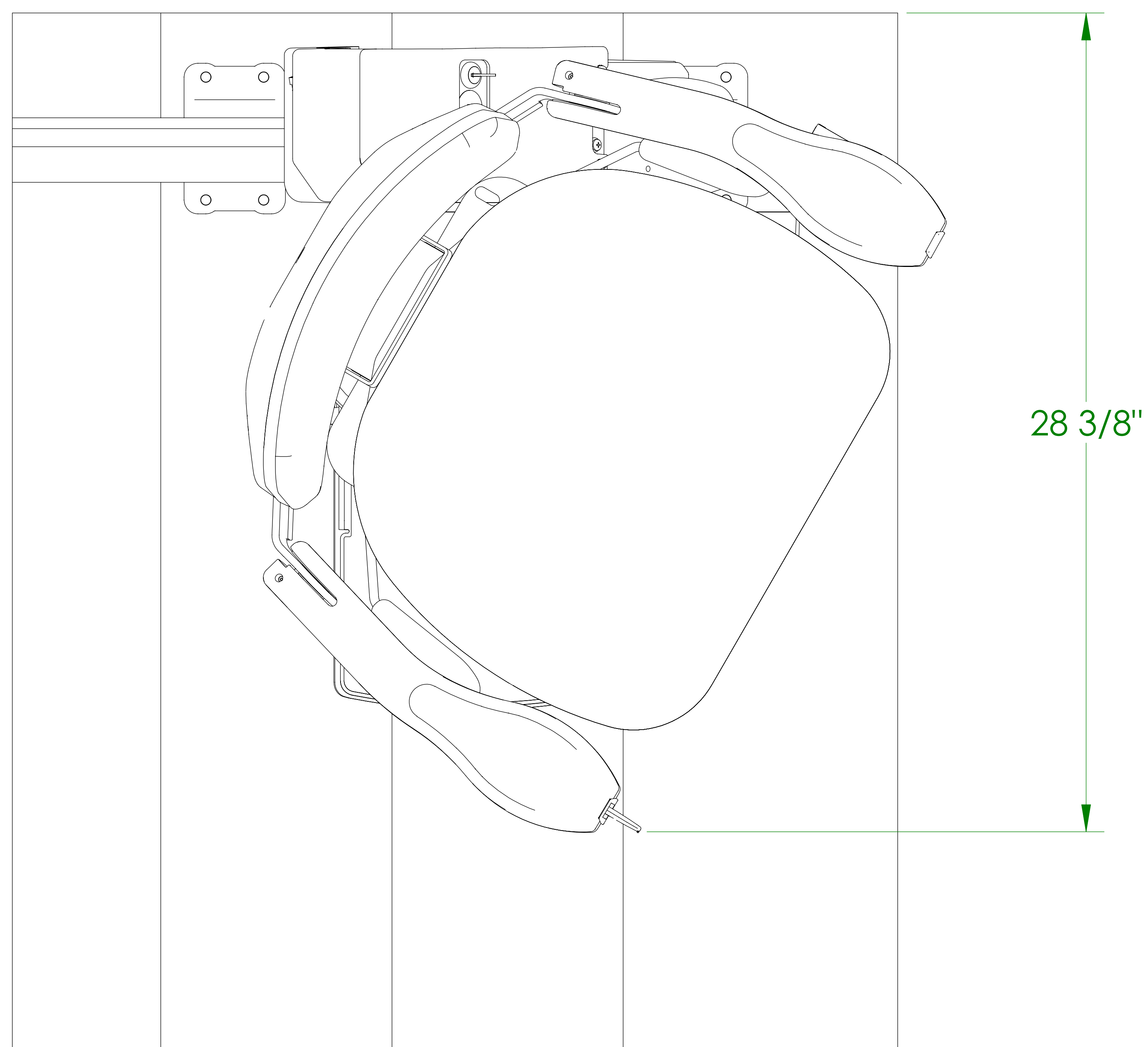
SEAT SWIVELED 60°
