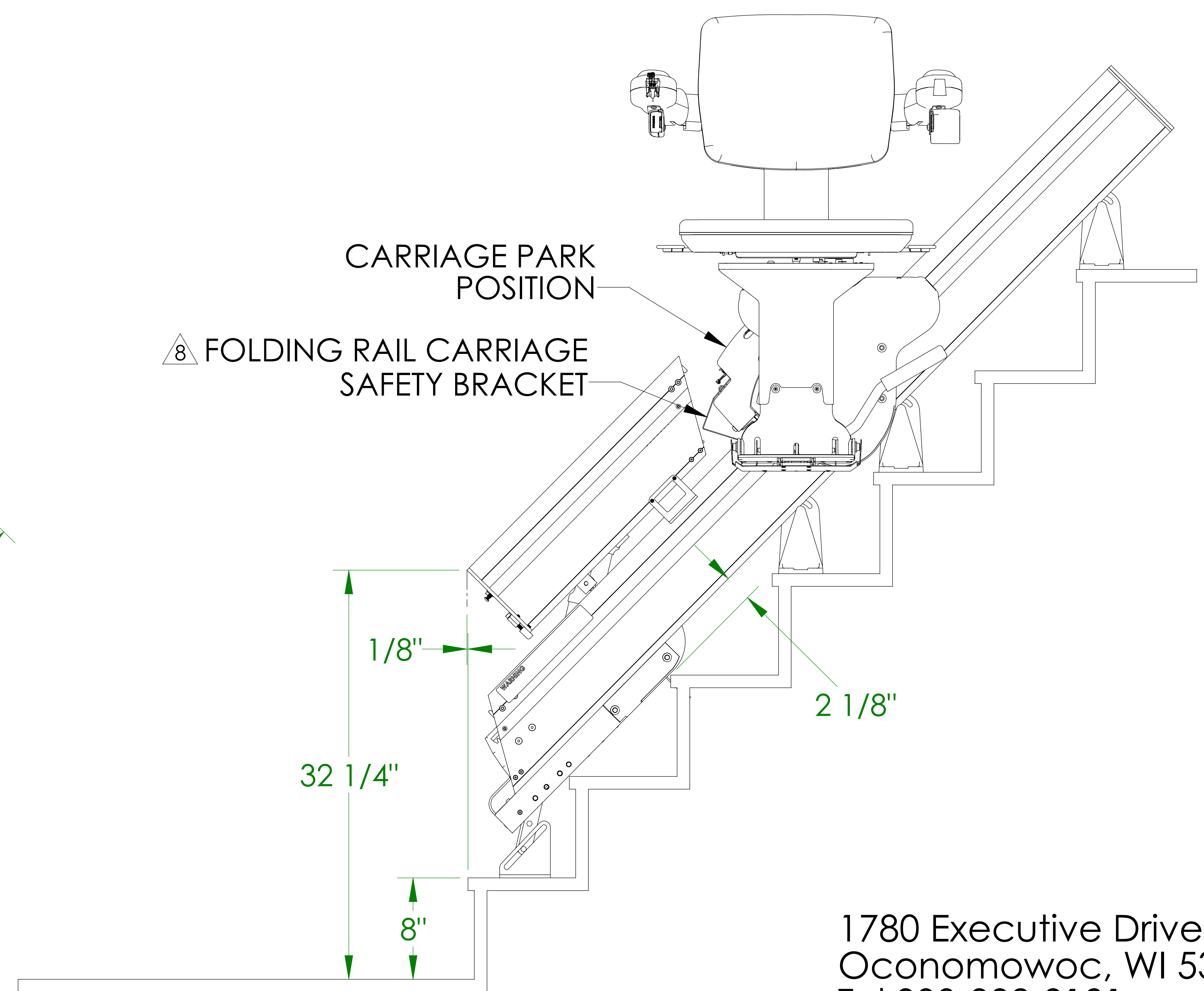
AUXILIARY ELEVATION VIEW RAIL FOLDED UP POSITION
