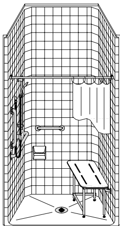
PERSPECTIVE VIEW - N.T.S. MODEL SHOWN HERE AS: LEFT PLUMBING RIGHT SEAT
