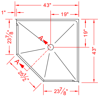
TOP VIEW - SCALE 3/8" = 1'-0"
