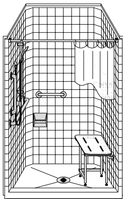
PERSPECTIVE VIEW - N.T.S. MODEL SHOWN HERE AS: RIGHT SEAT
