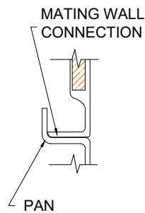
DETAIL PJ - SCALE: 3" = 1'-0" PAN JOINT DETAIL
