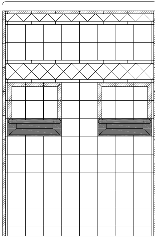
BACK WALL
